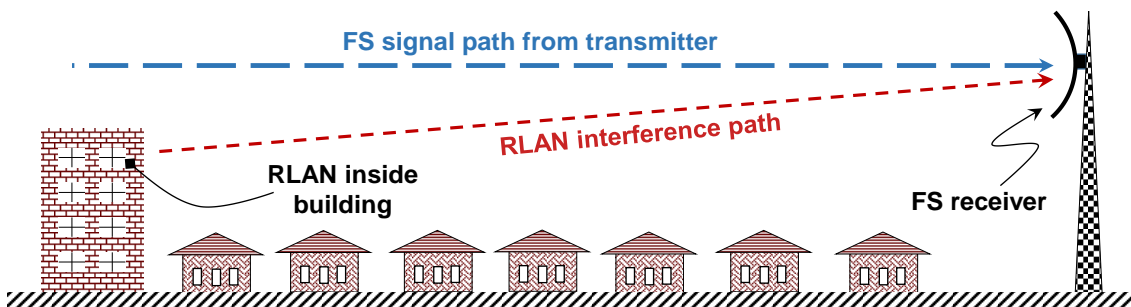
Figure 3: RLAN interference from indoor operation building (horizontal scale compressed)
