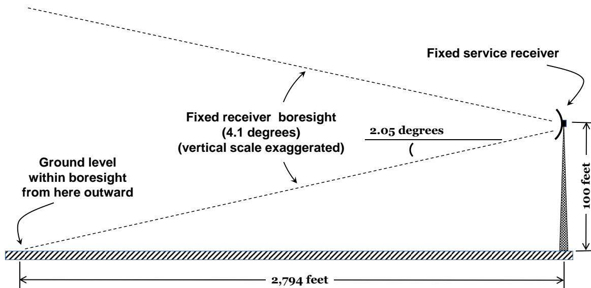
Figure 2: FS receiver boresight reaches ground level 0.53 miles from 100 ft. tower
